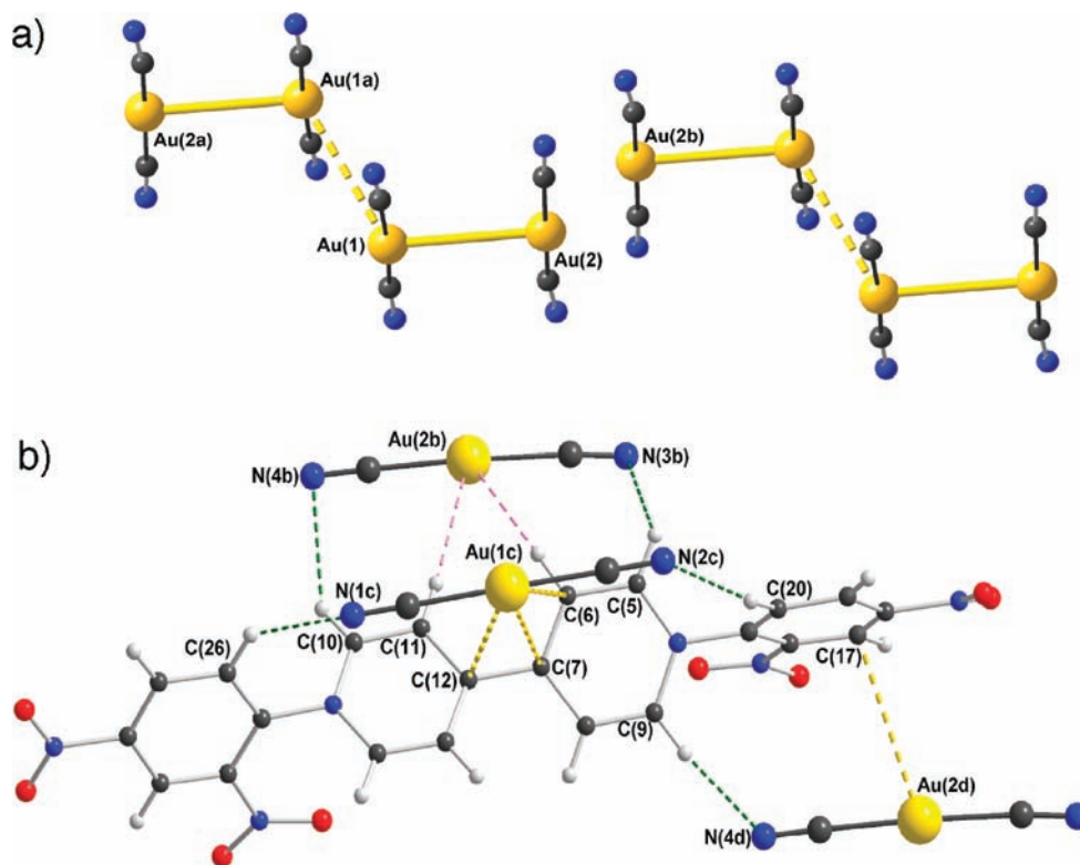
Figure 3. (a) Interactions between the dicyanoaurate complexes in 1 : Au(1)···Au(2) 3.5108(7) Å, Au(1)···Au(1a) 3.8738(9) Å, Au(2)···Au(2b) 4.7681(9) Å, Au(1a)···Au(1)···Au(2) 116.69(2)° (above). (b) Interactions between the DNP 2+ viologen cation and neighboring dicyanoaurate complexes; CH···N hydrogen bonds shown in green, C···Au contacts in the range 3.60–3.75 Å in yellow, H···Au contacts under 3.25 Å in pink (below). Symmetry codes: a \{-x, -y+1, -z+2\} ; b \{-x, -y+1, -z+1\} ; c \{x, y, z-1\} ; d \{-x+1, -y+1, -z+1\} .
