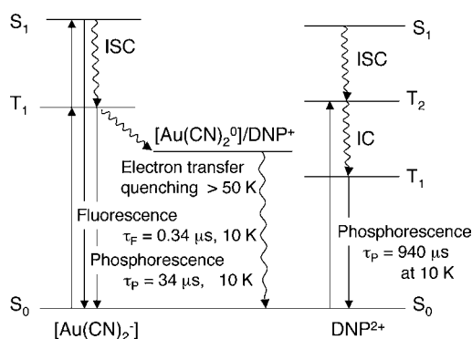
Figure 8. Energy diagram of the two emissive species. At higher temperature electron transfer quenches the [\text{Au}(\text{CN})_2]^- centered luminescence. S_0 , ground state; S_1 , first excited singlet state; T_1 , T_2 , first and second triplet states; IC, internal conversion; ISC, intersystem crossing.
