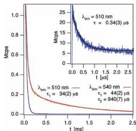
Figure 6. Luminescence decay curves of \{[\text{Au}(\text{CN})_2]_2\text{DNP}\} \cdot 4\text{H}_2\text{O} at T = 10 K for excitation at 355 nm with detection at 510 nm (blue), and 540 nm (red). Inset: expanded view of the first 2.5 \mu\text{s} for detection at 510 nm.
